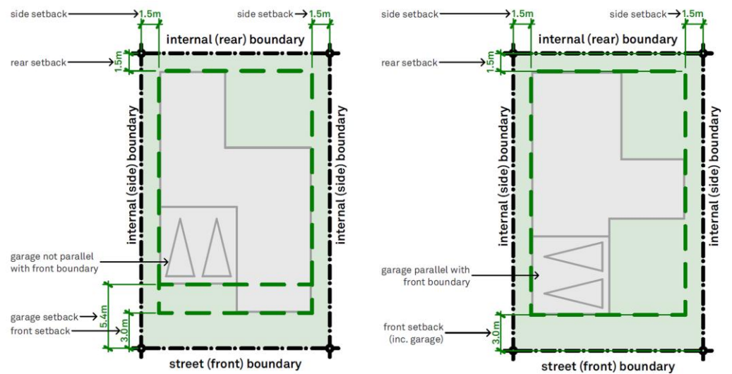
Diagram C3.4.2 – Positions of garage that comply with front yard setback in Residential Growth Precinct
