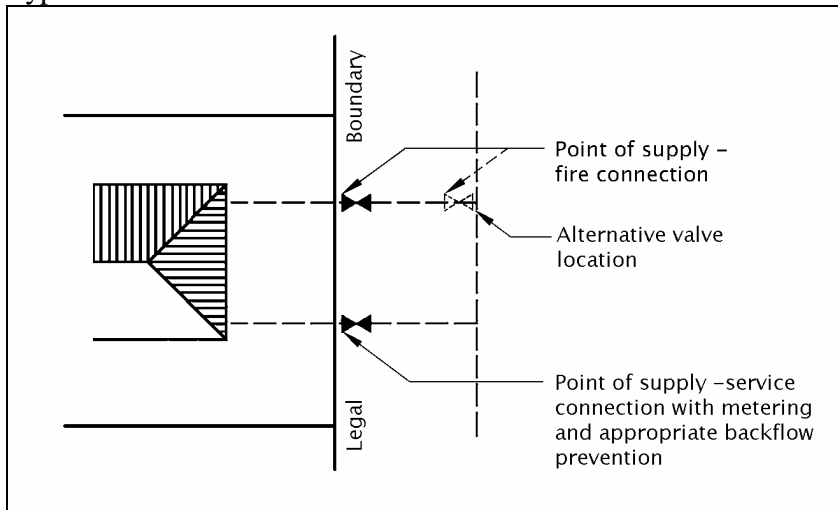
Type 1: Combined fire and service connection
